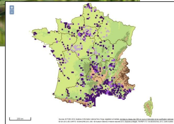
Vicia tetrasperma (L.) Schreb. subsp. gracilis (DC.) Hook.f. [LR BZH (NT)] (ph. RR)
